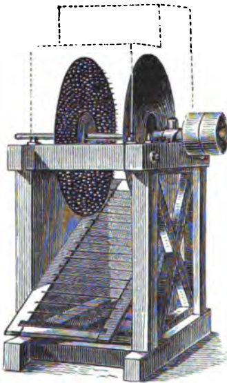
Fig. 401.—Mill for tearing up peat.
